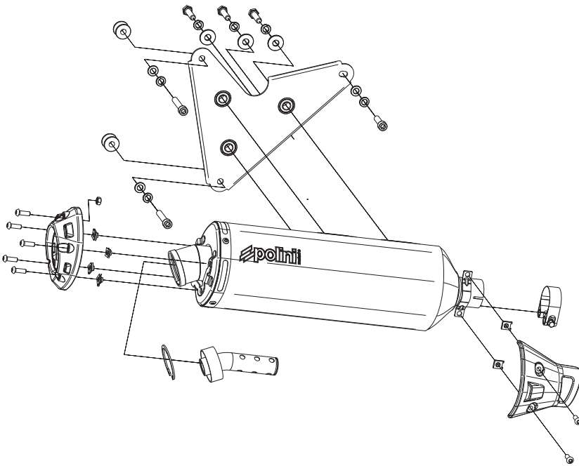
Silencer
